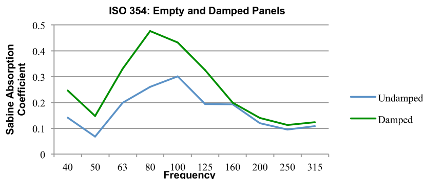
Figure 4: Absorption characteristics of damped and undamped panels as measured by ISO354
