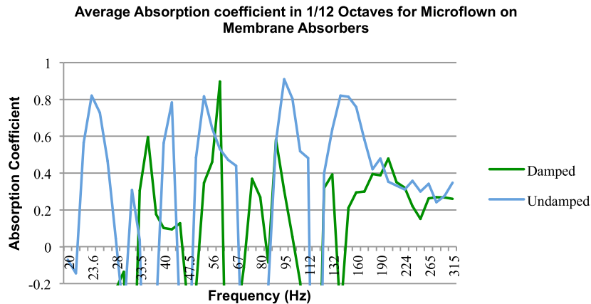
Figure 7: Average absorption coefficient for Microflow + Subwoofer for Membrane Absorber. In 1/12 Octave bands.
