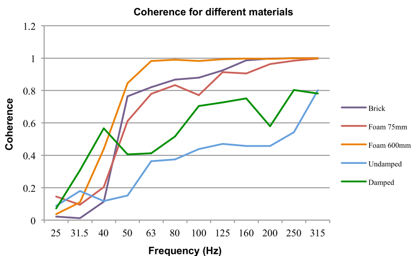
Figure 8: Coherence – comparison of different materials
