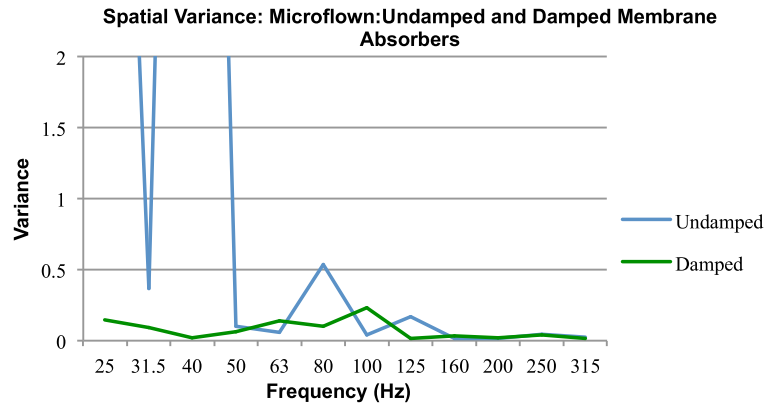
Figure 6: Spatial variance of Microflow + Subwoofer measurements for the membrane absorber
