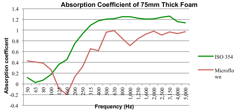
Figure 2: Absorption coefficients for 75mm thick foam measured by BS354 and by Microflown
