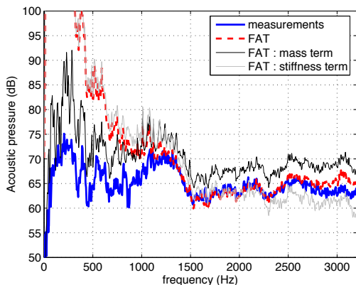
Figure 5: Measured and identified acoustic pressures averaged over the 16 array positions.
