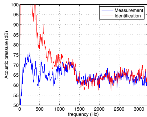
Figure 4: Measured and identified acoustic pressures for the first array position.
