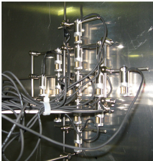
Figure 3: 13 microflow array designed for FAT applications.
