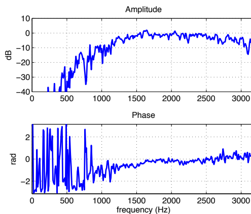
Figure 7: Transfer function H1 between measured and identified acoustic pressures.
