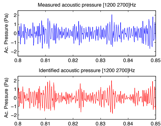
Figure 6: 50ms of measured and identified acoustic pressures in the time domain. Band pass filter [1200 2700Hz].
