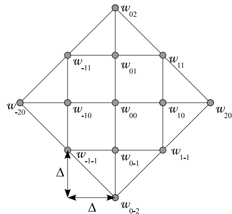
Figure 1: 13 measurement grid required to apply the FAT at the central point w_{00}
