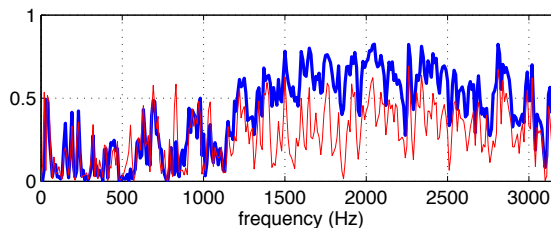
Figure 8: Coherence functions between measured and identified acoustic pressures (blue thick line), and between measured acoustic pressure and plate velocity at the same point (red thin line).
