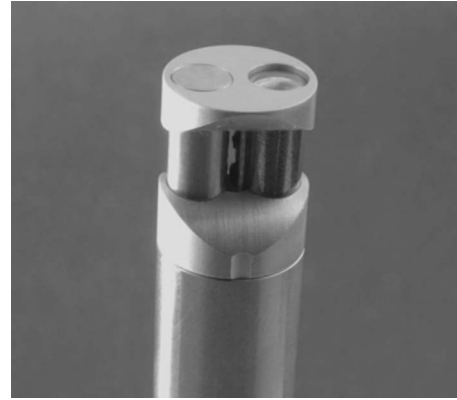
FIG. 2. A Microflow 1/2 in. sound intensity probe. The particle velocity sensor can be seen on the solid cylinder to the right; the electret microphone is mounted inside the other cylinder.
